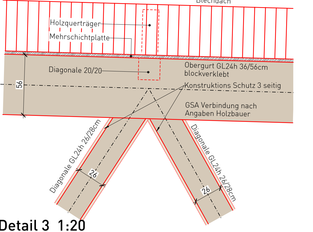
Detail 3 1:20
