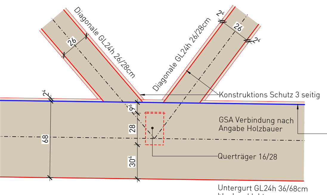
Detail 2 1:20
