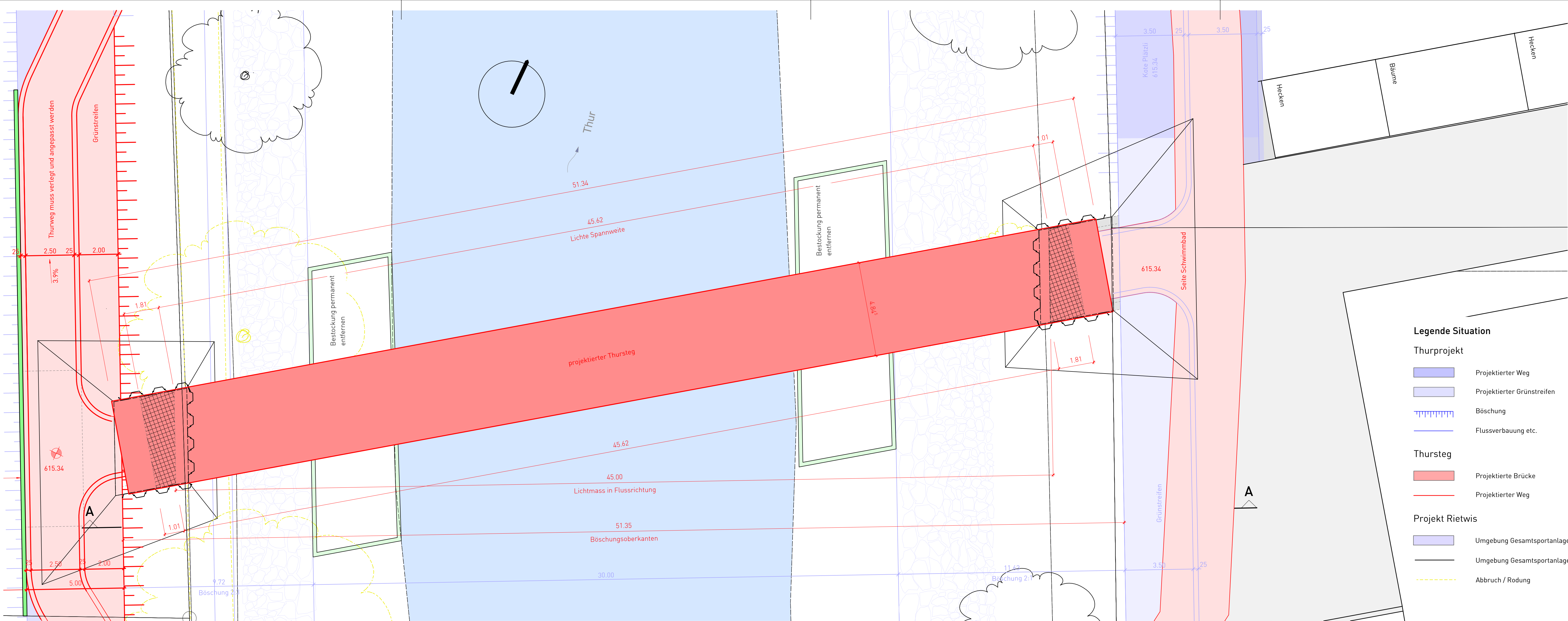
Situation 1:100
