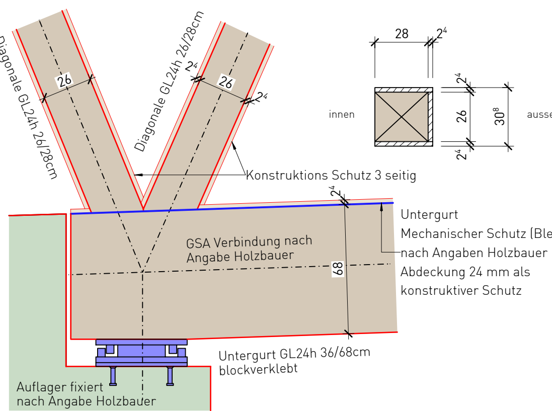
Detail 1 1:20
